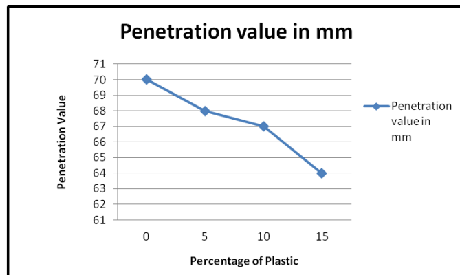
Figure 8 Variations in Penetration Value of Bitumen with Increase in percentage of plastic
